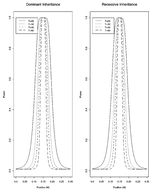
Figure 5 Power curves of the test statistics F_{AB,ad} against the position of markers at 0.01 significant level for a mode of dominant inheritance a = d = 1.0 , and a mode of recessive inheritance a = 1.0, d = -0.5 , respectively. The QTL locates at 15 cM which is flanked by two markers A and B . Here the mutation age T = 20, 30, 40, 60 , and the other parameters are the same as those in Figure 4.
