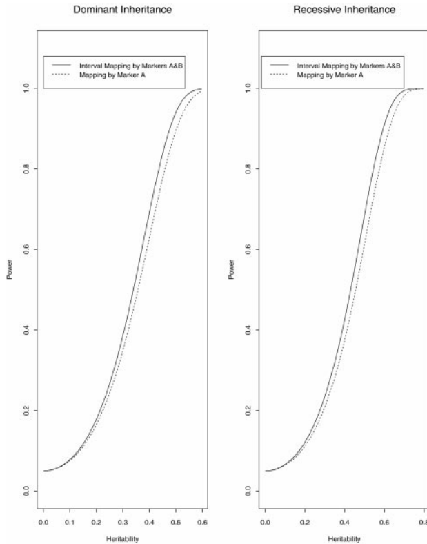
Figure 6 Power curves of the linkage interval mapping by markers A and B , and linkage mapping by marker A against the heritability h^2 , when q_1=p_A=p_B=0.50 , \lambda_{AB}=30 cM, \lambda_{AQ}=\lambda_{QB}=15 cM, k=250 , \sigma_{G_a}^2=0.10 , \sigma_{G_d}^2=0.05 , at 0.05 significant level for a mode of dominant inheritance a=d=1.0 , and a mode of recessive inheritance a=1.0 , d=-0.5 , respectively.
