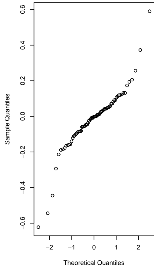
Normal Q-Q Plot
