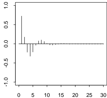
C . Partial Correlogram
