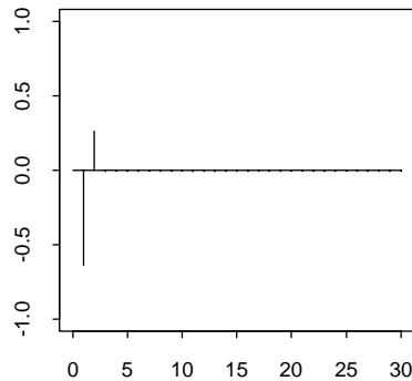
G . Partial Correlogram
