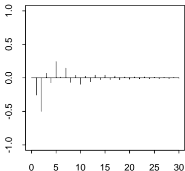
B . Partial Correlogram
