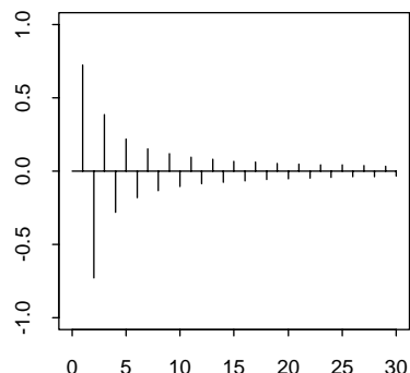
D . Correlogram, R(0) = 7.39
