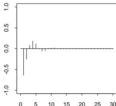
H . Correlogram, R(0) = 16.96
