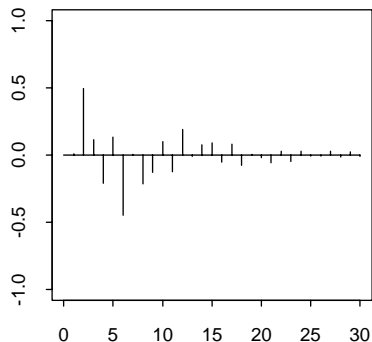
F . Partial Correlogram
