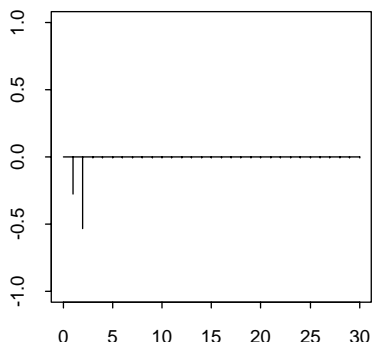
B . Correlogram, R(0) = 1.61
