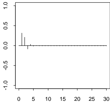
E . Partial Correlogram
