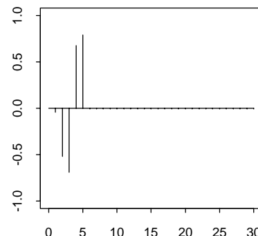
J . Correlogram, R(0) = 4.6
