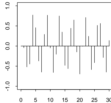
I . Partial Correlogram
