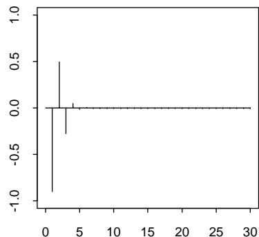
D . Partial Correlogram
