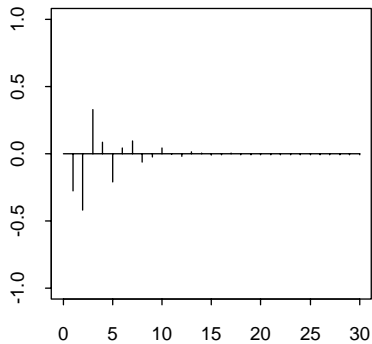
A . Partial Correlogram
