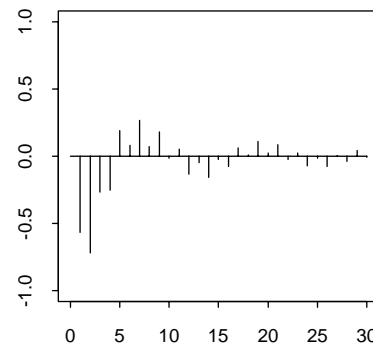
J . Partial Correlogram
