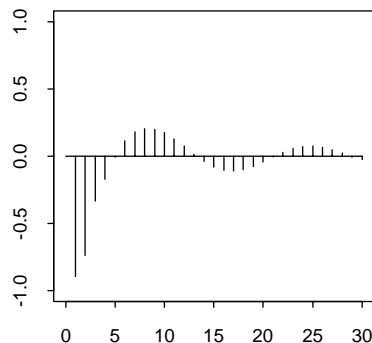
H . Partial Correlogram
