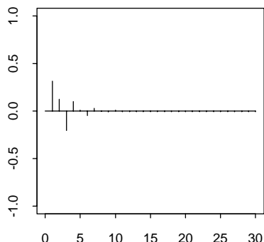
F . Correlogram, R(0) = 2.12
