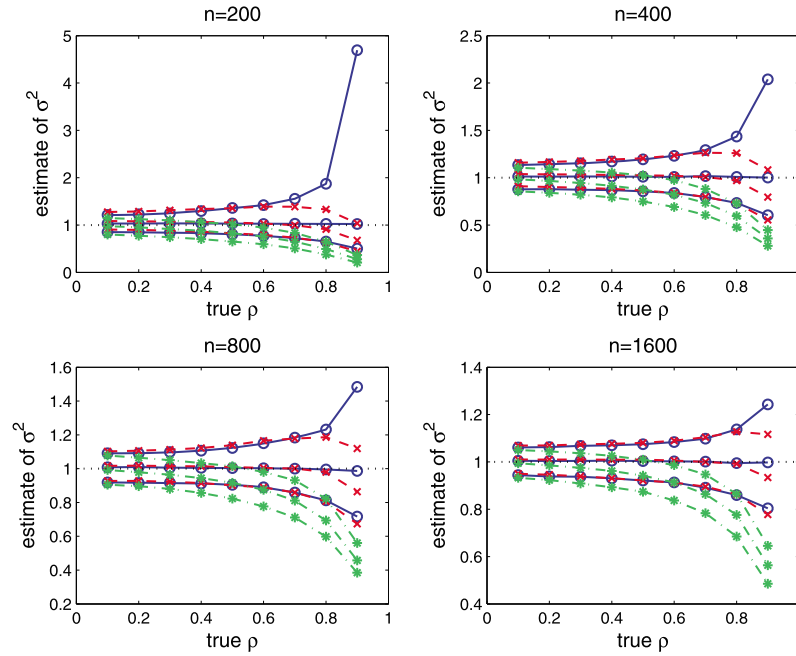
Figure 1. Experiment of Section 3.1: plots of the 5th, 50th and 95th sample percentiles of estimators of \sigma^2 : our variogram estimator (—○—), the Hall and Van Keilegom estimator of [7] (---x---) and the Tong and Wang estimator of [15] (*--*--*). The true \sigma^2 is 1 (···). The trend is g(x) = 10 + 12.5x^3(1 - 0.5x)^3 .
