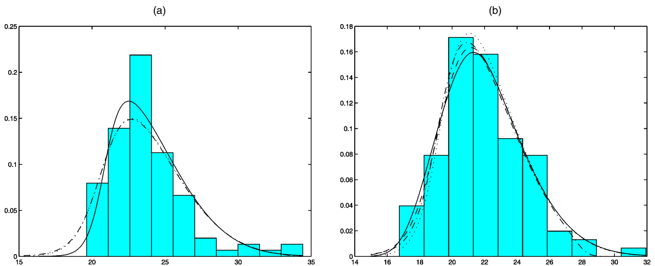
Figure 3. Histograms of 102 Male (a) and 100 Female (b) Australian Athletes' BMIs and pdf's Using Different Posited Skewing Functions. The skewing functions are \pi_1 and \pi_3 (whose nuisance parameters are estimated through minimizing estimation variance) and \pi_{1m} and \pi_{3m} (whose nuisance parameters are estimated through MLE) [· · · \pi_1(x) ; · · · \pi_3(x) ; - - \pi_{1m}(x) ; — \pi_{3m}(x) ]. In (a), the two pdf's using \pi_{1m} and \pi_{3m} overlay each other and are indistinguishable.
