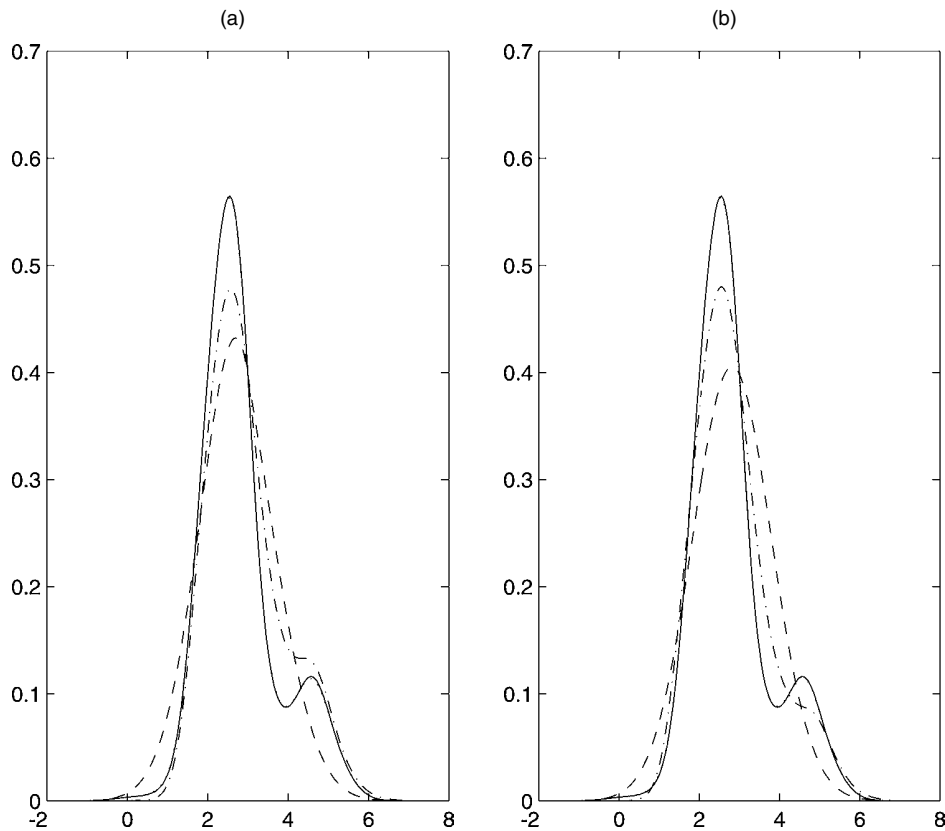
Figure 1. The Average Estimated pdf's Using the Posited Models \pi_1 , \pi_3 , and \pi_t [— \pi_0(x) ; - - \pi_1(x) ; · · · \pi_3(x) ; ··· \pi_t(x) ]. The true pdf using \pi_0 and the average estimated pdf using \pi_t overlay each other and are indistinguishable in these plots. The nuisance parameters in the posited models are selected to minimize the resulting variance (a), and are estimated using MLE (b). The sample size is 500, and 1,000 simulations were done.
