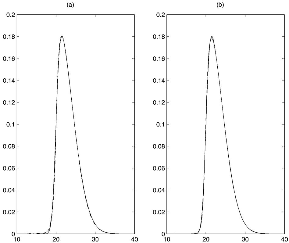
Figure 2. The Average Estimated pdf's Using the Posited Models \pi_1 , \pi_3 , and \pi_t [— \pi_0(x) ; - - \pi_1(x) ; · · · \pi_3(x) ; · · · \pi_t(x) ]. The curves are very close to each other and are indistinguishable. The nuisance parameters in the posited models are selected to minimize the resulting variance (a), and are estimated using MLE (b). The sample size is 100, and 1,000 simulations were done.
