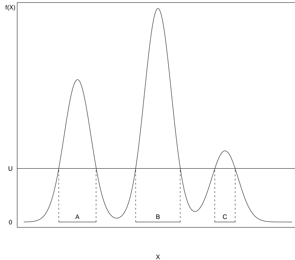
Figure 1: The slice sampler for a multimodal distribution: Draw X|U uniformly from the sets labeled by A , B and C .
