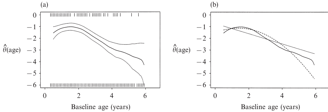
Fig. 1. (a) Estimated kernel estimate \hat{\theta}(\text{age}) when fitting the semiparametric model to the infectious disease data assuming working independence. Also displayed are 95% pointwise confidence intervals: solid line, \hat{\theta}(\text{age}) ; dotted lines, 95% CI. The vertical strokes at 0 and -6 indicate the occurrence of 1 and 0 in the response. (b) Comparison of the kernel estimate \hat{\theta}(\text{age}) and the estimated linear and quadratic baseline age models: solid line, kernel estimate; dotted line, linear estimate; dashed line, quadratic estimate.
